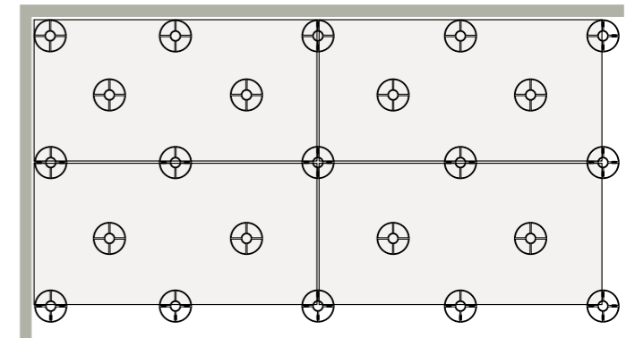
Posa sopraelevata 60x120 ± 2 cm 24"x48" ± 3/4" Installation onto flat surfaces (raised laying)
